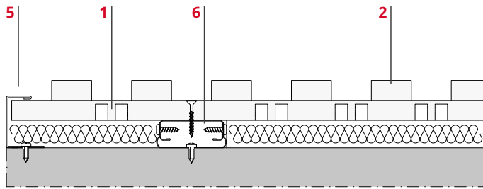
FINITURA LATERALE (A) LATERAL FINISHING (A)
