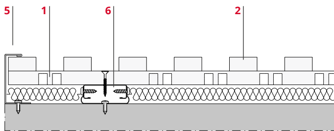
FINITURA LATERALE (B) LATERAL FINISHING (B)
