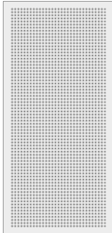
IS 3.10/16 Forate passo 16 mm parallelo Ø 3+10 mm Perforated 16 mm parallel pitch Ø 3+10 mm
