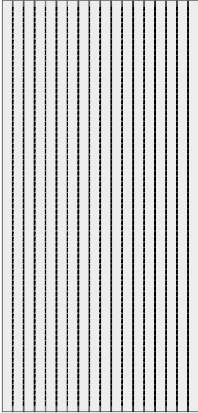
IS 29.3 Fresate 3 mm passo 32 mm Retro forato Ø 10 mm – Passo 32X16 mm 3 mm grooves 32 mm pitch Holes Ø 10 mm – 32X16 pitch
