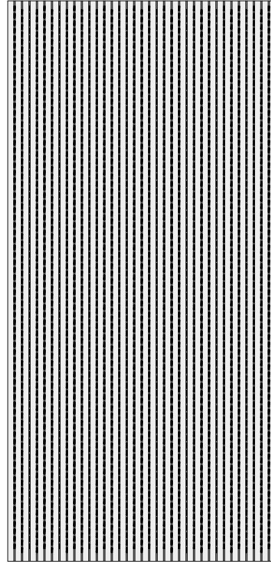
IS 13.3 Fresate 3 mm passo 16 mm Retro forato Ø 10 mm – Passo 16X16 mm 3 mm grooves 16 mm pitch Holes Ø 10 mm – 16X16 pitch
